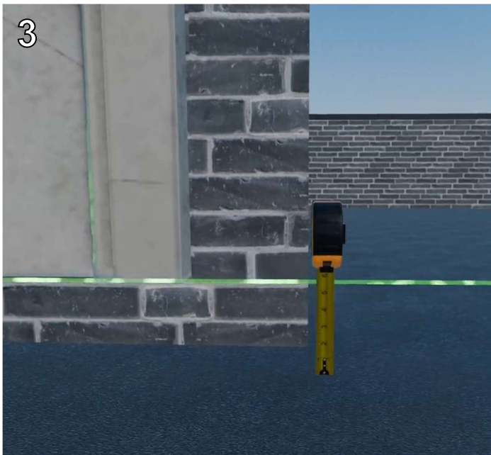
Verify slope of roof deck and all adjoining floors & doorways to ensure correct pedestals were ordered to reach desired finish floor height. Refer to provided Mbrico project shop drawings for pedestal key and color-coded pedestal layout map.
