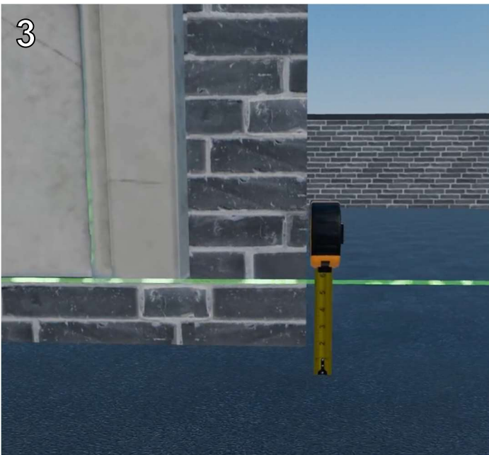
Verify slope of roof deck and all adjoining floors & doorways to ensure correct pedestals were ordered to reach desired finish floor height. Refer to provided Mbrico project shop drawings for pedestal key and color-coded pedestal layout map.
