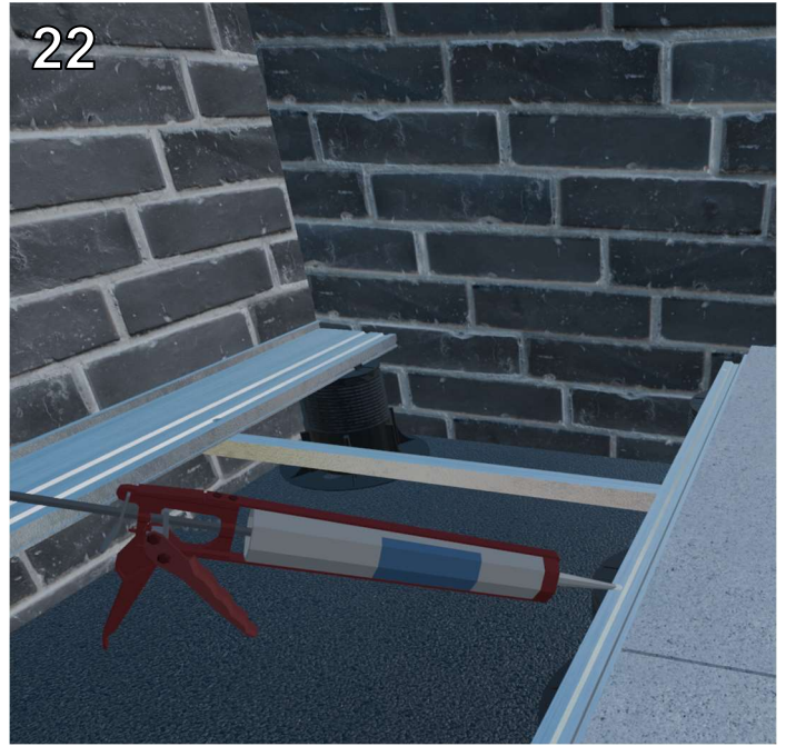
22 Place dabs of provided Mbrico adhesive onto the track where all four corners of tiles will sit on tracks.
