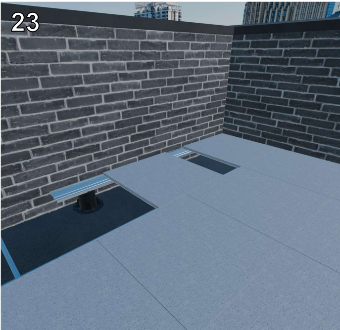
23 Slide tile from track end into designated location. Repeat previous step and this step to complete this segment of tracks.
