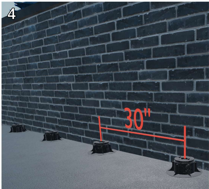
Place first row of pedestals, per provided project layout, at your designated starting edge. Refer to provided Mbrico shop drawing suggested control/starting point for your project. Place pedestals 30" on center.
