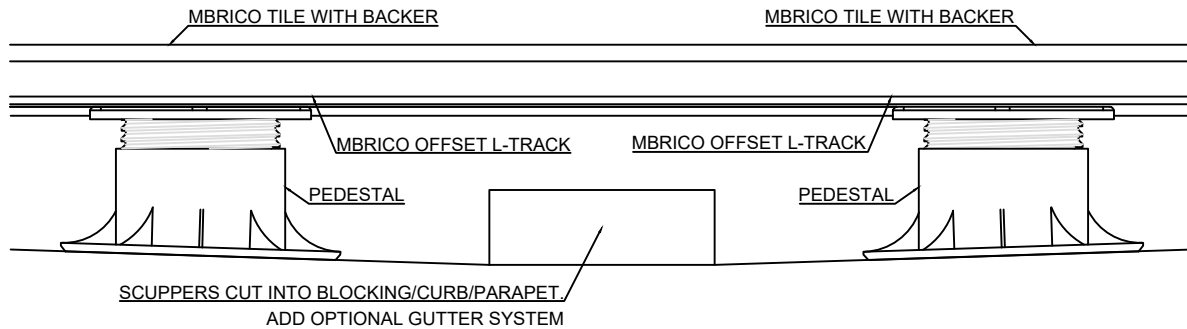
DETAIL FRONT VIEW
