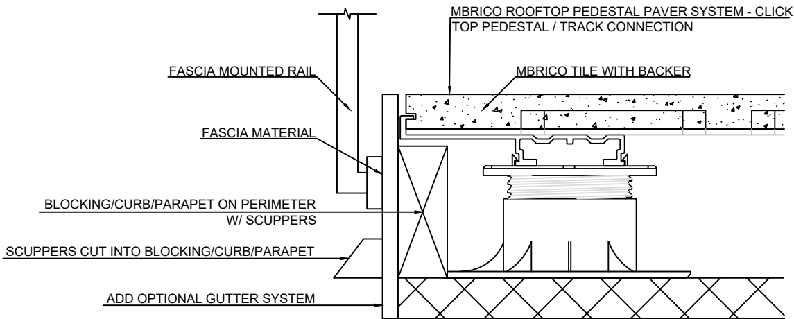
DETAIL SIDE VIEW
